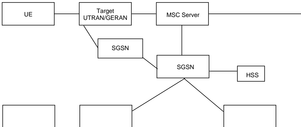
Figure 5.13a: SRVCC architecture for UTRAN (HSPA) to 3GPP UTRAN/GERAN with Gn based SGSN
